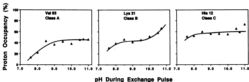
FIG. 3. pH profile for labeling by a 37-msec pulse applied 400 msec after initiation of refolding. The pH profiles are presented for three amide protons, each representative of one of the three major groups of amide protons, which are classified according to both the pH profile and the kinetics of acquisition of protection from exchange (see text and Table 1). The time constant for exchange of a free peptide amide proton is 2 msec at pH 9 and 10°C, but the inductive effect of side chains and neighboring residues may make exchange more than 10-fold faster (8). A decrease in labeling from a plateau level is seen at pH values below 9. This is the result of exchange being base catalyzed: as the pH during exchange is decreased, the duration of the pulse (37 msec) starts to limit complete labeling of an unprotected amide hydrogen site. The pH of the exchange pulse was varied between pH 7.6 and 11 by changing the composition and pH of the exchange buffer. Mops was used as the buffer below pH 8.5, and glycine was used for the higher pH values.
