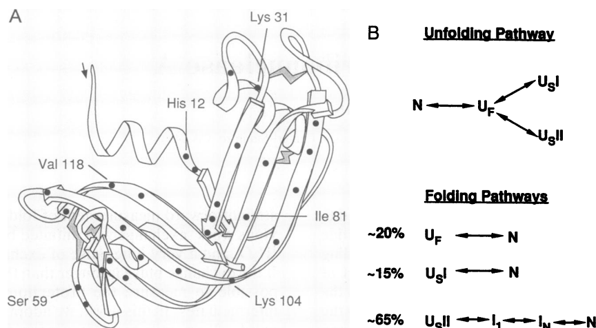
FIG. 1. (A) Location of amide protons used as structural probes to investigate the folding pathway of RNase A. Some have been labeled on this ribbon diagram of the protein (diagram courtesy of Jane Richardson), so that others may be identified from the complete list in Table 1. Helix 1 encompasses residues 3–13; helix 2, residues 25–34; and helix 3, residues 50–60. Approximately 40 amide protons are stable to exchange with ^2\text{H}_2\text{O} in native RNase A, under the conditions of recording of a correlated spectroscopy (COSY) NMR spectrum. Of the 40 amide protons, only 27 could be used as probes for folding; the NMR resonances of the others were either too weak or showed overlap under our spectrum recording conditions. (B) Pathways of unfolding and folding of RNase A. Unfolded RNase A (U) is kinetically heterogeneous: it consists of a mixture of a fast-folding species, U F (20%), and at least two slow-folding species, U S I (15%) and U S II (65%) (5), each of which folds to native RNase A (N) by an independent pathway. A native-like intermediate, I N , had previously been identified on the folding pathway of U S II. I N differs from N by the same isomerization that differentiates U S II from U F , probably (6) a trans isomer of Pro-93 in I N versus a cis isomer in N. I 1 is a hydrogen-bonded intermediate formed on the folding pathway of U S II within 100 msec (see text and Fig. 2), which is likely to be on the direct pathway of folding. I N is not formed on the unfolding pathway of N. The scheme for the refolding of U S II that is shown is the simplest possible minimal model that can account for the data.
