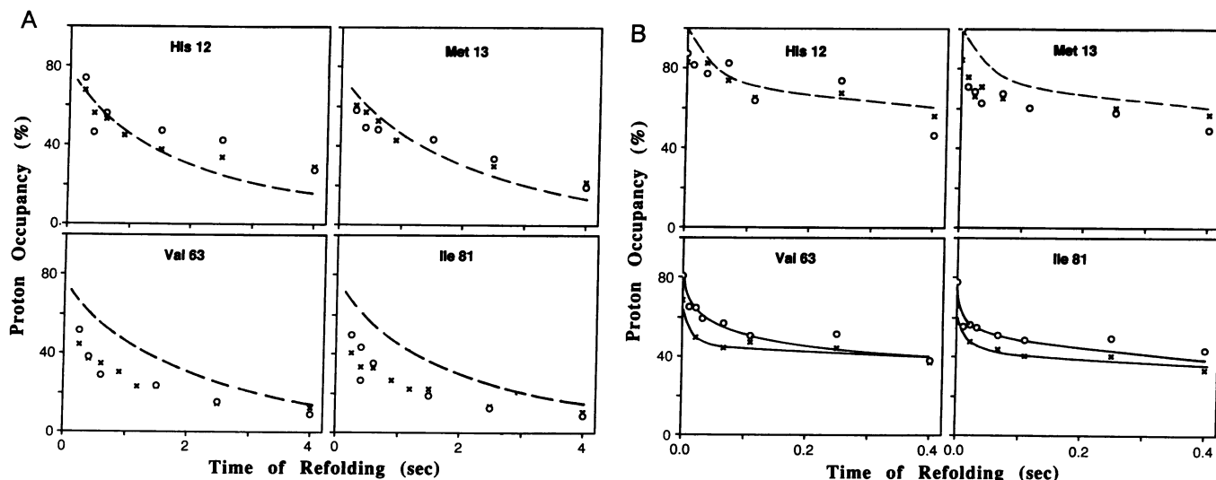
FIG. 2. Acquisition of protection of backbone amide deuterons from exchange with solvent protons. The proton occupancy of a backbone amide hydrogen site, in a COSY NMR spectrum, is a measure of the extent of labeling by exchange (proton incorporation) at that site and is plotted versus time after initiation of refolding for four different amide protons and on two different time scales: 0–4 sec (A) and 0–400 msec (B). The pH during the exchange pulse was 9 (x) or 10 (o). The dashed lines indicate the progress of the refolding reaction monitored by measuring the accompanying change in tyrosine absorbance at 287 nm and correspond to the formation of I_N from U_{SII} (Fig. 1B). The other lines through the data points were drawn by inspection only.
