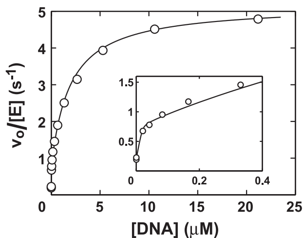
FIGURE 3. Dependence of the observed ATP hydrolysis rate constant ( v_o/[E] ) of Y782F topoisomerase II (15 nM) on the concentration of the 68-bp DNA duplex with saturating (3 mM) Mg^{2+} -ATP. The line represents a fit of the data to Scheme 1.
