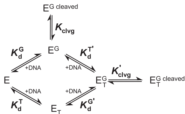
SCHEME 2 DNA cleavage reaction
