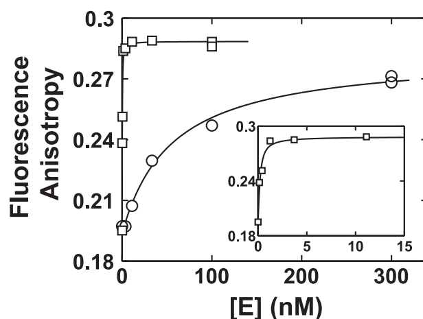
FIGURE 5. Equilibrium fluorescence anisotropy measurement of wild-type and Y782F mutant topoisomerase II to a fluorescently labeled 40-bp DNA duplex (see supplemental Table S1 for sequence). The indicated concentrations of wild-type (○) and Y782F mutant (□) enzyme were used to titrate 0.8 and 0.16 nM DNA, respectively. Fitting the data to quadratic binding isotherms (Equation 2; lines) gave apparent binding affinities for the wild-type and mutant enzymes of K_{d, \text{wild type}} = 60 nM and K_{d, \text{Y782F}} \leq 0.14 nM, respectively. The apparent DNA affinity for the mutant enzyme is an upper limit, because the DNA concentration employed in this experiment (0.16 nM) is similar to the apparent affinity.
