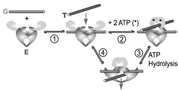
FIGURE 1. Proposed mechanism of topoisomerase II catalyzed DNA transport (2, 3). G, G-DNA; T, T-DNA; E, topoisomerase II (ATPase domains are colored light gray). Steps 1–4 are described in the Introduction.
