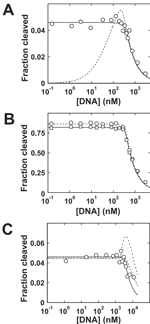
FIGURE 4. Equilibrium DNA cleavage mediated by topoisomerase II as a function of the total concentration of a 46-bp DNA duplex (see supplemental Table S1 for sequence). A , DNA titration of 360 nM topoisomerase II in the presence of 10 mM Mg^{2+} and 0.5 mM AMPPNP. Data points are averages from triplicate measurements. The data are fit to a model in which enzyme bound to a single DNA is competent to cleave DNA ( K_{clvg} > 0 ; Scheme 2, solid line ) and to a model in which T-DNA is required for DNA cleavage ( K_{clvg} = 0 ; dashed line ). As a side condition for the fits, the absence of observed DNA binding cooperativity was assumed as indicated from the analysis of the ATPase data (Table 2). Also, to demonstrate consistency of the data with a higher affinity of the G-DNA site relative to the T-DNA site, K_d^G < K_d^T was used as a side condition for the fit shown by the solid line . B , DNA titrations of 360 nM topoisomerase II in the presence of 10 mM Ca^{2+} ( \square ) or 10 mM Ca^{2+} and 0.5 mM AMPPNP ( \circ ). Lines are fits of the data to models in which K_{clvg} is allowed to exceed 0 and K_d^G < K_d^T , as in A . C , DNA titration of 3200 nM topoisomerase II in the presence of 10 mM Mg^{2+} and 0.5 mM AMPPNP. Data points are the averages of duplicate measurements. The lines are fits of the data to Scheme 2 for ratios of K_{clvg}^G to K_{clvg}^T of 1 ( solid line ), 5 ( dashed line ), 7.5 ( dotted line ), and 10 ( dashed and dotted line ). The probability p(\chi^2) that a particular model can fit the
