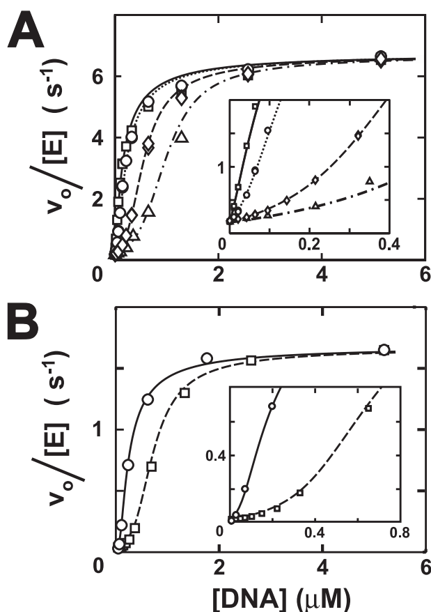
FIGURE 2. Dependence of the observed ATP hydrolysis rate constant ( v_o/[E] ) on the concentration of the 68-bp DNA duplex at varying concentrations of topoisomerase II with saturating (A; 3 mM) or subsaturating (B; 60 \mu\text{M} ) \text{Mg}^{2+} -ATP. Enzyme concentrations were as follows: 13 nM ( \square ), 65 nM ( \circ ), 325 nM ( \diamond ), and 650 nM ( \triangle ) (A) and 400 nM ( \square ) (B). The lines represent a global fit of the data to Scheme 1.
