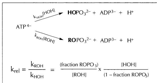
Fig. 4. Partitioning of phosphoryl transfer between water and alcohol.
