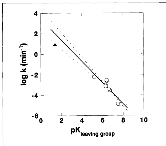
Fig. 7. Dependence of the hydrolysis of phosphoanhydrides on leaving group pK a . Data are from Table 2. The upper dashed line of slope -1.2 is a least-squares fit to the circles (○), representing reactions involving leaving groups of the type: -OP(O) 2 Y. The closed triangle (▲) corresponds to the reaction in which diethylphosphate [-OP(O)(OR) 2 ] is the leaving group [7]; its inclusion in a least-squares fit gives the lower dashed line of slope -0.9. The slopes of these lines are taken to be outer limits for \beta_{\text{leaving group}} , and their average is represented by the solid line of slope \beta_{\text{leaving group}} = -1.1 . The conclusions drawn in the text do not change depending on which of these slopes is used to represent \beta_{\text{leaving group}} .
