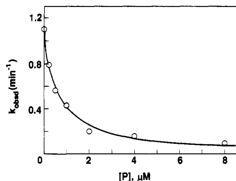
FIGURE 4: Dependence of k_{\text{obsd}} on the concentration of the product inhibitor, \text{pppG}_2\text{CCCGCU} . The reaction of \sim 1 \text{ nM } p^*G_2\text{CCCGCUA}_5 and 800 \mu\text{M G} catalyzed by 50 \text{ nM} ribozyme at 50^\circ\text{C} in 50 \text{ mM} MES, pH 7, and 10 \text{ mM} \text{MgCl}_2 . The line is the best fit to the data for K_i = [E][I]/[E \cdot I] = 0.6 \mu\text{M} and competitive inhibition such that the E \cdot I complex is totally inactive.
