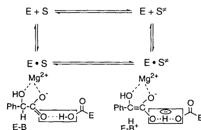
Fig. 1. A simplified illustration of the proposal of LBHB participation in enzymatic catalysis, showing proton abstraction catalyzed by mandelate racemase. An LBHB between the carboxyl oxygen and Glu 317 on the enzyme would stabilize the enolate intermediate or transition state (2, 3). Bond notation in boxes: (···) represents the normal, weak H bond in the ground state (E-S) with unmatched pK_a 's; (—) and the intermediate position of the proton represent the strong LBHB formed in the transition state (E-S*) when their pK_a 's become matched. Ph, phenyl.
