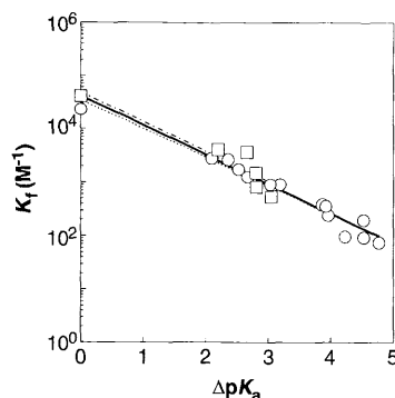
Fig. 3. Formation constants of the H-bonded complexes of substituted phenols with 3,4-dinitrophenolate (circles) or 4-nitrophenolate (squares) in THF as a function of \Delta pK_a^{\text{water}} . The solid line represents the overall fit of the data for both series with \beta = 0.65 ; the lighter dashed lines represent the fit of individual series of data for H bonding with 3,4-dinitrophenolate ( \beta = 0.63 ) or 4-nitrophenolate ( \beta = 0.65 ). The \Delta pK_a values in water were used because the values in THF have not been determined. These \Delta pK_a^{\text{water}} values are expected to be proportional to those in THF (38–40, 43), but the range of \Delta pK_a is expected to be >10 in THF (42). Data are from Table 3.
