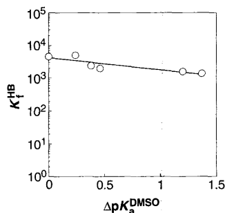
Fig. 2. Formation constants of the intramolecular H bonds as a function of \Delta\text{p}K_a^{\text{DMSO}} for a series of substituted phthalate monoanions in DMSO [ \beta = 0.37 with the \Delta\text{p}K_a^{\text{DMSO}} scale, or \beta = 0.9 with the \Delta\text{p}K_a^{\text{water}} scale (not shown)]. Data are from Table 2.
