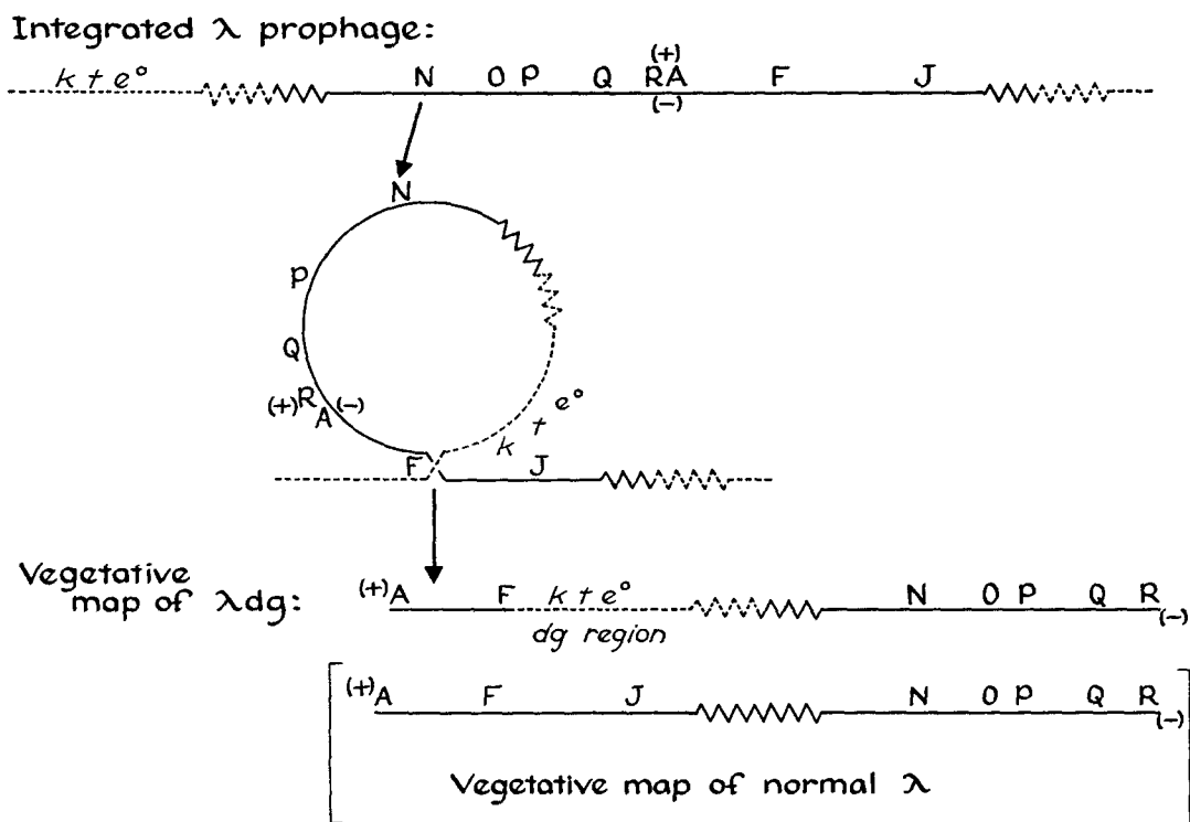
FIGURE 2. Formation of lambda dg from prophage. The symbols are those defined in Fig. 1. Independent isolates of lambda dg are different in respect to the left-hand end point of the dg region, which is defined by both the extent of the deficiency in lambda genes and the extent of addition of E. coli genes. Starting at and always including the K, L, I, J group, the deficiency can extend to the left to a varying extent, in some cases including the entire A -to- M group (see Fig. 1) (7). The amount of the galactose operon added in lambda dg can also vary, the excluded portion always extending from the left-hand end of k to the right into t (18); however, most lambda dg contain the entire operon. To comply with these facts the model must allow for variation in the position of the crossover that will yield closed forms of differing size.
