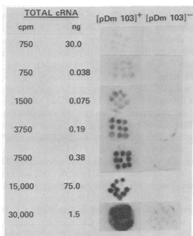
FIG. 3. Hybridization of different amounts of pDm103 [ 32 P]cRNA to [pDm103] + and [pDm103] - colonies. Colonies were obtained by transferring HB101 [pDm103] or HB101 bacteria, respectively, to 13-mm filters with toothpicks. In the experiments where \leq 1.5 ng of cRNA were applied per filter, the specific activity = 2 \times 10^7 cpm/ \mu g. The lower specific activities used for the other two experiments were obtained by mixing this cRNA with unlabeled pDm103 cRNA. The weak response observed for [pDm103] - colonies could result either from E. coli DNA impurities in the pDm103 DNA preparations used to prepare the [ 32 P]cRNA, or from some similarity of sequence in pDm103 and E. coli DNAs.
