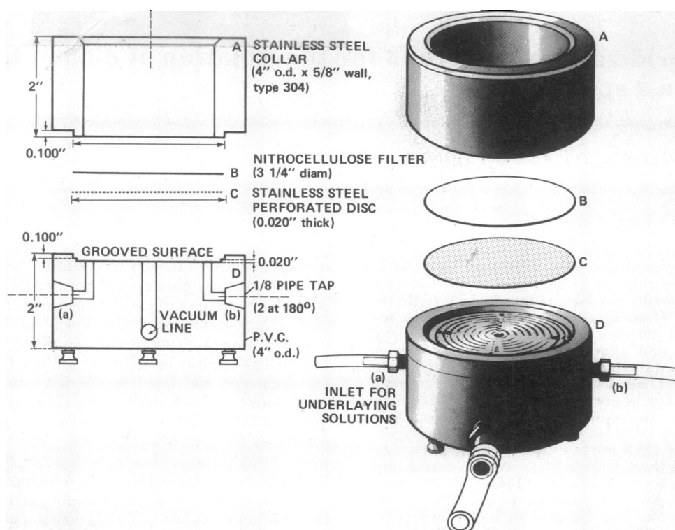
FIG. 1. Apparatus for treatment of colonies on filters. To wet the underside of the filter, solutions are introduced through ports (a) or (b), while the tube connected to the vacuum port is clamped off. Solutions are removed through the vacuum port which is connected to a water aspirator. Other procedures are described in the text. ", inches (2.54 cm); o.d., outside diameter; P.V.C., polyvinyl chloride.
