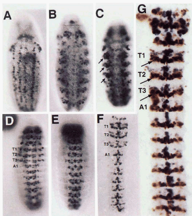
FIGURE 3.—Expression of neryy during embryogenesis. All panels are photomicrographs of embryos (A–E) or dissected nerve cords (F and G) stained for neryy RNA; anterior is up. (A) neryy expression began in a subset of neuroblasts in stage 9 embryos. (B) In stage 10 embryos, neryy expression appeared to be excluded from the CNS and may be limited to the peripheral nervous system (PNS). No segmental differences in neryy expression were apparent at these early stages. (C) In stage 11 embryos, neryy expression in thoracic segments (arrows) was elevated relative to its expression levels in abdominal segments. (D) In late stage 12 embryos (close to the end of germ band shortening) neryy expression close to the ventral midline was observed. At this stage, the thoracic segments (T1–T3) express neryy in additional, more laterally positioned cells than abdominal segments (e.g., A1). (E) After germ band shortening is complete (stage 14) neryy expression again appeared identical in all thoracic and abdominal segments. (F) In a dissected nerve cord from a stage 15 embryo clear differences in the neryy expression pattern were again visible in thoracic and abdominal segments. (G) A dissected stage 15 nerve cord stained for neryy RNA and en protein (brown). The additional thoracic-specific neryy -positive cells also expressed en (arrows).
