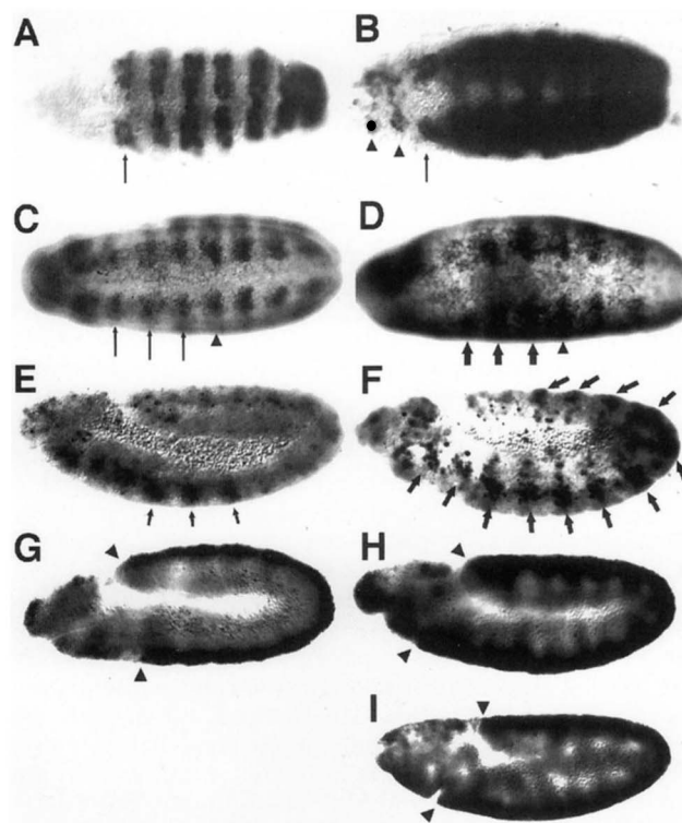
FIGURE 1.— lips , 412, belt , and nervy are induced by ubiquitous UBX expression during embryogenesis. HS:Ubx-FS (A, C, E, and G), HS:Ubx (B, D, F, and H), and HS:Antp (I) stage 11 embryos stained for 412 (A,B); lips (C and D); nervy (E and F); and belt (G–I) RNA by in situ hybridization. The embryos in A–D are ventral views of germband elongated embryos, therefore only anterior segments are visible; the remaining panels are lateral views. At this stage, 412 RNA is present in the mesoderm of PS2 to PS14 (the arrows in A and B point to PS2 expression). After ubiquitous UBX expression (B), 412 expression is highly induced in PS2 to PS14. In addition, two additional anterior parasegments PS0 and PS1 express 412 (B, arrowheads). At stage 11, lips was expressed in two patches of ectodermal cells per segment and the three thoracic segments expressed lower levels (C, arrows). After ubiquitous UBX expression, the level of lips RNA was elevated in the three thoracic segments (D, arrows). The arrowheads in A and B point to lips expression in the first abdominal segment (A1), which appeared the same. nervy was expressed in nervous system precursor cells in head, thoracic, and abdominal segments and the three thoracic segments expressed higher levels (E, arrows). Elevated levels of nervy RNA were observed in all segments in response to ubiquitous UBX expression (F, arrows). belt was expressed at uniform levels throughout the germ band from T1 through A8 (the arrowheads in G mark the extent of this expression). Additional belt expression in the head was weaker and out of the plane of focus. Either ubiquitous UBX (H) or ubiquitous ANTP (I) expression induced ectopic belt expression anterior to T1 (the arrowheads in H and I mark the extended belt expression pattern).
