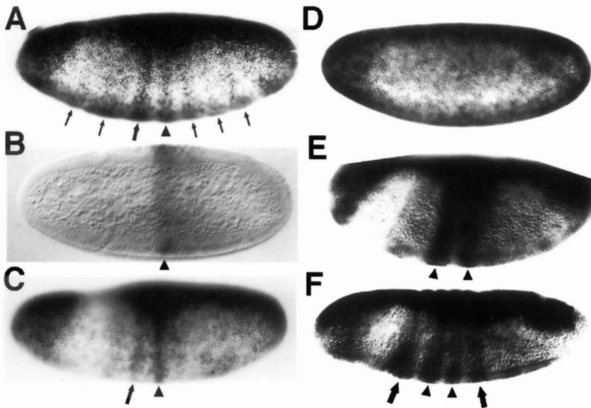
FIGURE 6.— lipis is regulated by homeotic genes very early in embryogenesis. (A) The wild-type lipis expression pattern during cellularization (stage 5). Expression was strongest along the dorsal surface and in two transverse stripes at 50% EL (arrowhead) and at 57% EL (thick arrow). In addition, weaker stripes are also visible (thin arrows). (B and C) Similarly aged embryos as in (A) but probed for Ubx expression (B) or both Ubx and lipis (C). One of the two strong stripes of lipis expression appeared to coincide with Ubx expression at this stage (arrowheads in B and C). The Ubx probe used in (B) was entirely derived from the 3'-most Ubx exon and therefore only identified mature or nearly mature transcripts. In Scr - Antp - Ubx - abd-A - Abd-B - stage 5 embryos (D) the stripes of lipis expression were not visible whereas the dorsal expression was unchanged. In wild-type stage 6–7 embryos, lipis expression was strongest dorsally and in two of the central lipis stripes; ubiquitous UBX-FS expression (E) did not alter this wild-type pattern. In contrast, ubiquitous UBX expression resulted in four strong stripes of lipis expression [F; arrowheads point to lipis stripes at 50 and 57% EL (also in E) and arrows point to an increase in lipis expression].
